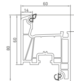
025 4 chamber sash
