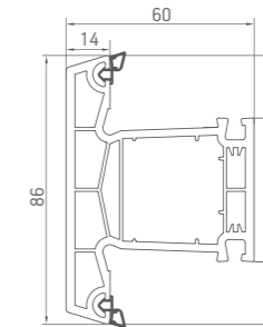
003 4 chamber mullion
