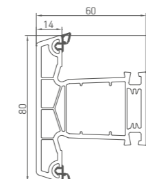
027 4 chamber mullion
