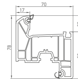
062 5 chamber sash
