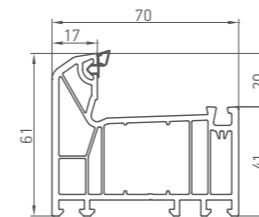
061 5 chamber frame
