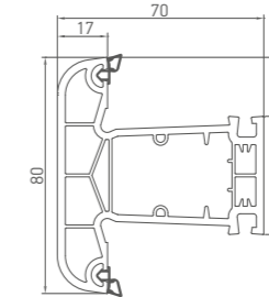
058 6 chamber mullion
