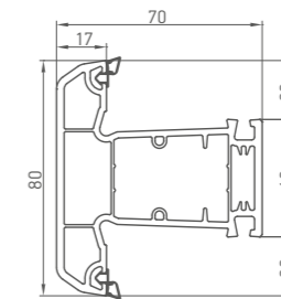
063 3 chamber mullion
